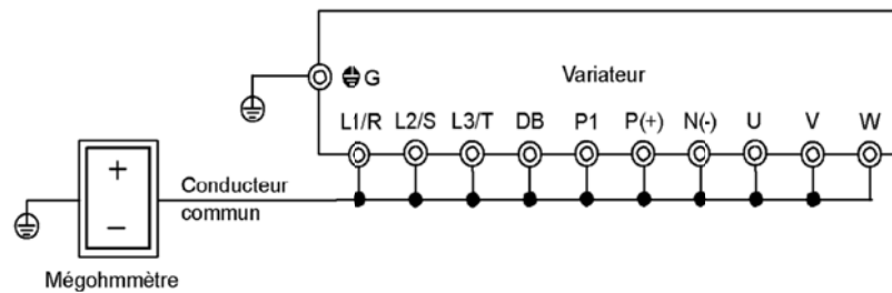
Figure 7-4-1 Test d'isolation
